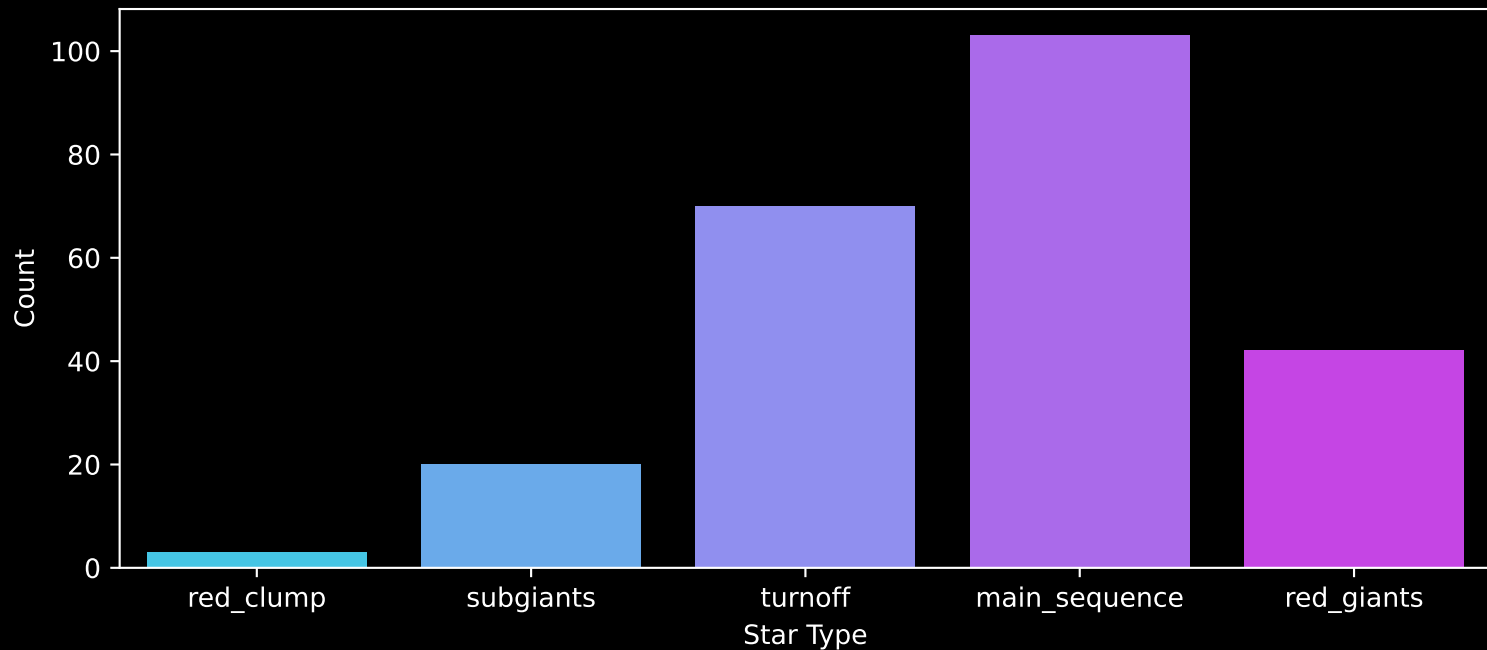
GALAH DR4 Field: [3168] Count plot of Star Type
