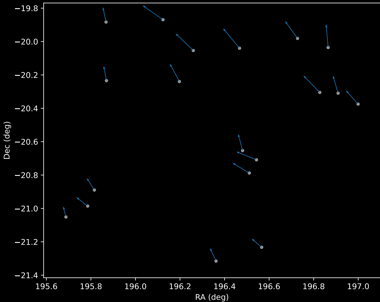
GALAH DR4 Cluster 0 Proper Motion Vectors (n=19)
