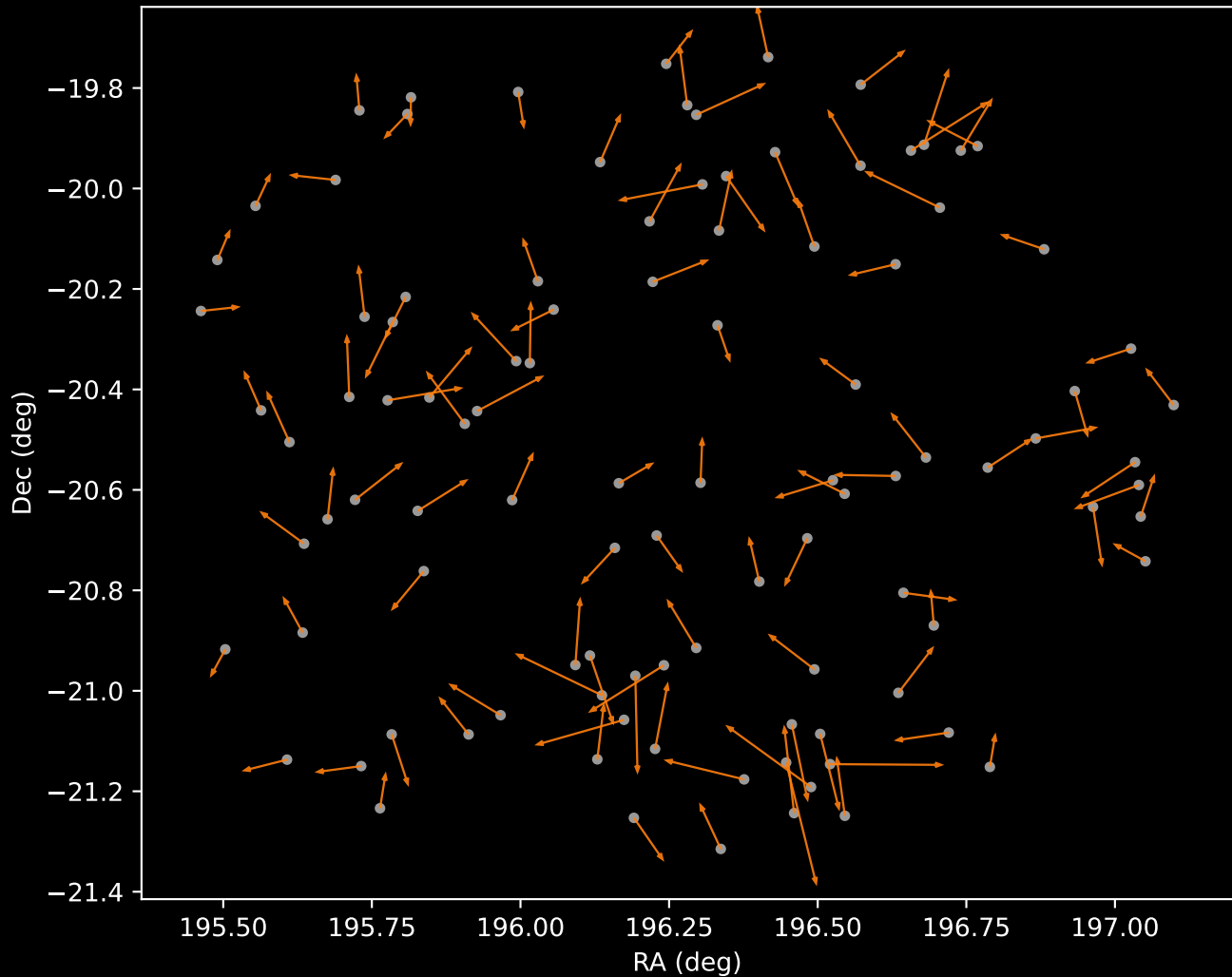
GALAH DR4 Cluster 2 Proper Motion Vectors (n=104)
