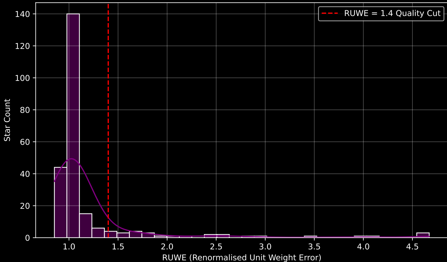
GALAH DR4 Field [3168] RUWE Distribution (n= 234)
